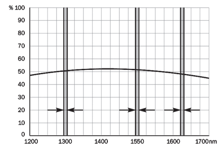
Wavelength dependence of Coupling Ratio of symmetrical SSCs at 1310nm, 1550nm und 1625nm
