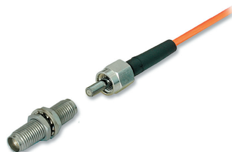
Standard F-SMA with 3.175mm hard metal ferrule.
